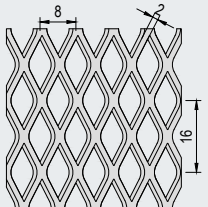
RB25 Open area: 50%
