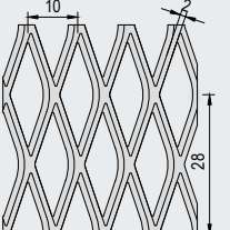
RB35 Open area: 58%
