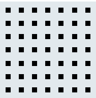
Unity 3 Square 3.5x3.5mm, c/c 8.3mm
