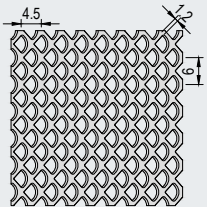
KD100 Open area: 35%
