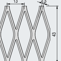
RB55 Open area: 62%
