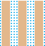
Unity 3 Perforation: Square 3.5x3.5mm, c/c 8.33mm Gypsum Strips: 12 strips, glued to perforated tile @ c/c 50mm
